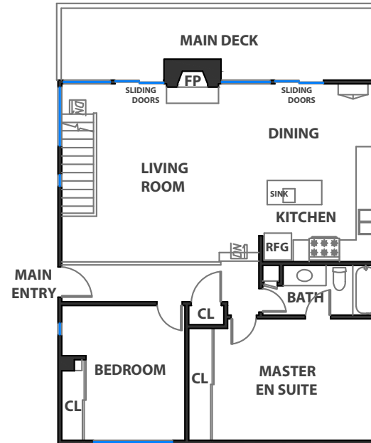
MAIN LEVEL
